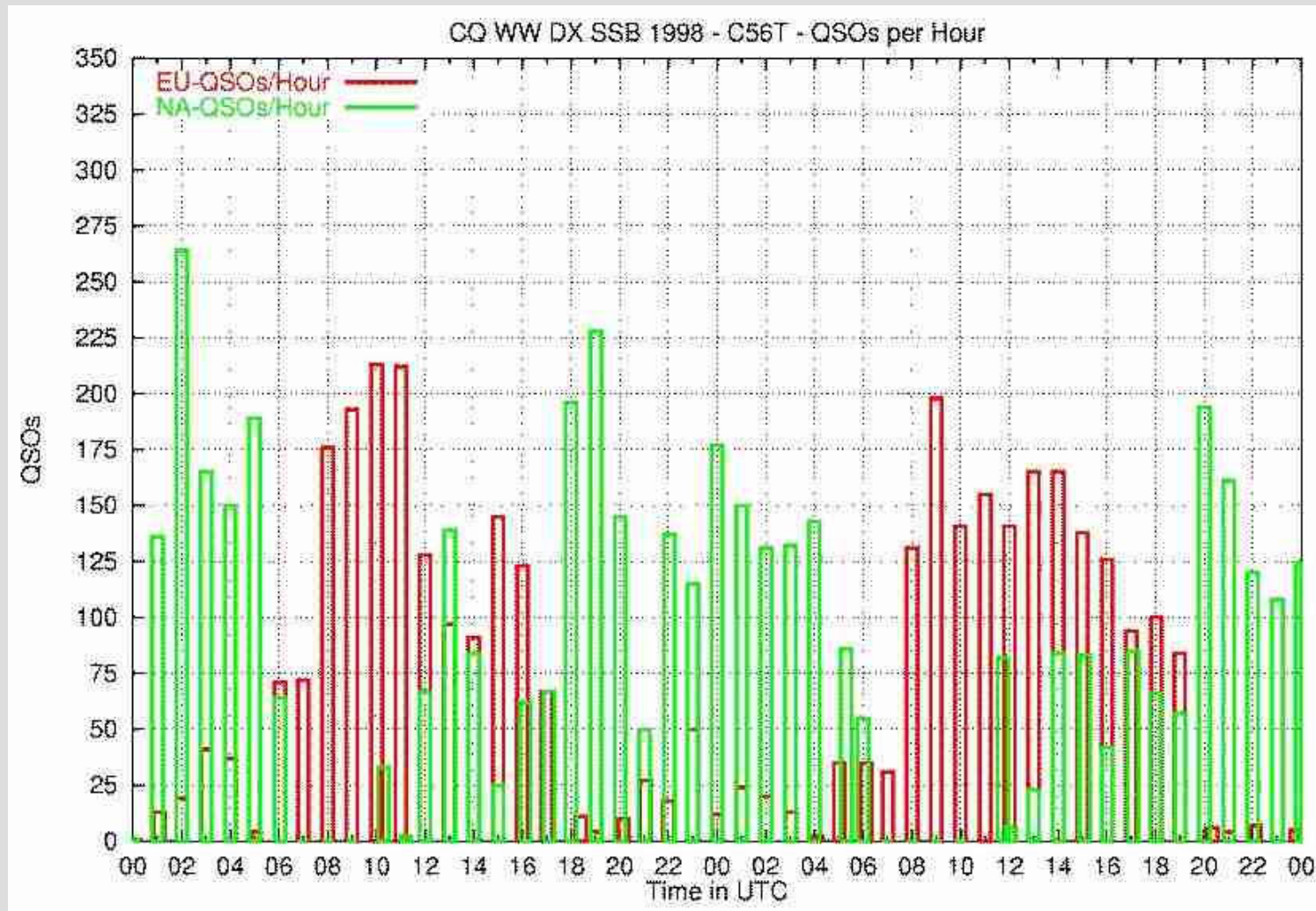
C56T: QSOs by hour, Europe red, North America green
